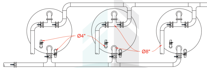
filter pipes details Scale : N.T.S
