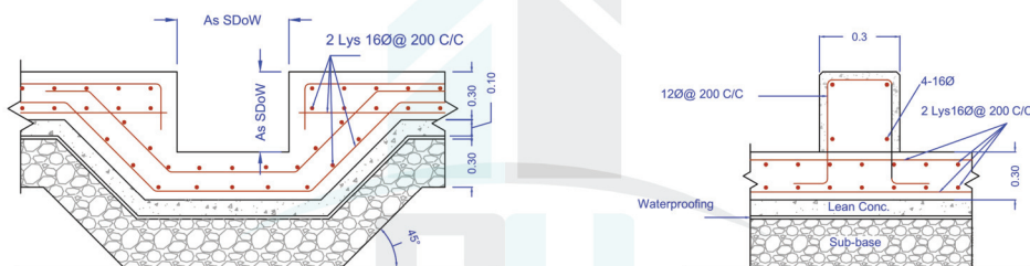
New Reinf. concrete Base, beams under tanks and Channel on new base - details
