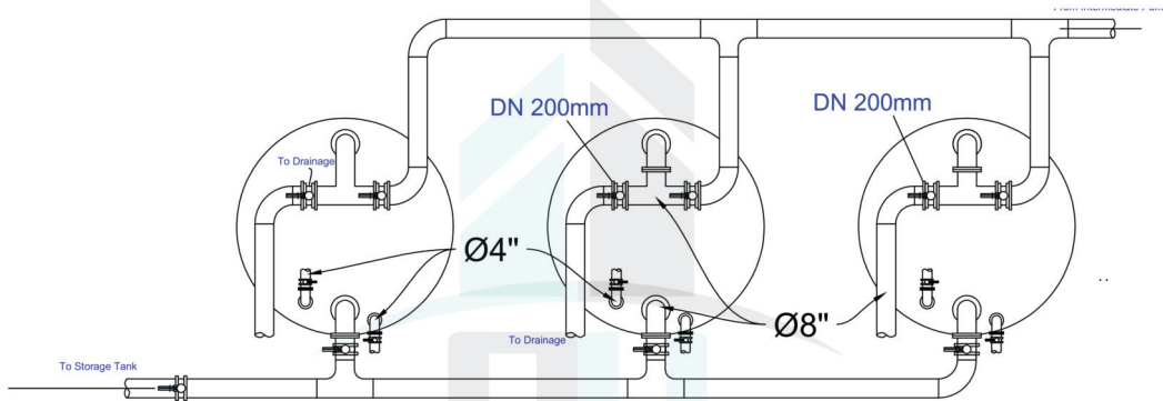
filter pipes details
